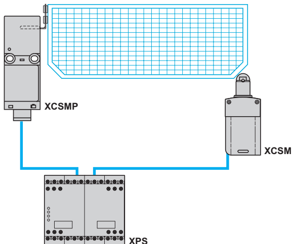
Locking of actuating key and operation in positive mode associated with a safety control unit.
